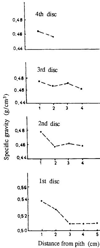
Fig. 1. Radial variation of specific gravity at four heights for Cupressus sempervirens based on 30 trees.
