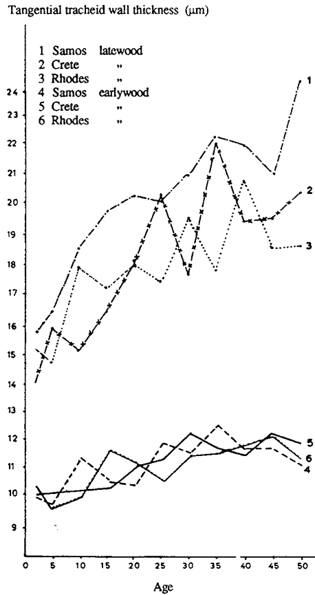
Fig. 12. Patterns of variation in tangential tracheid wall thickness of earlywood and latewood to ring number from the pith in the three provenances.
