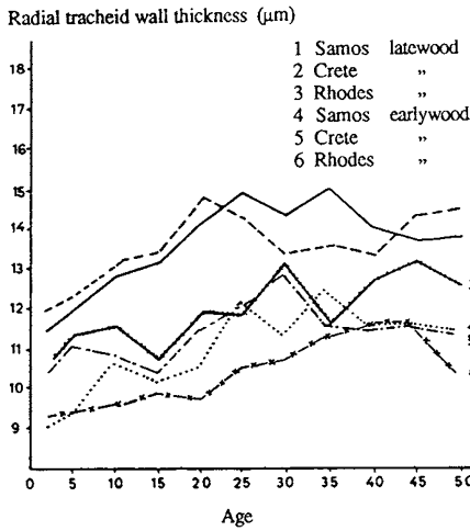
Fig. 11. Patterns of variation in radial tracheid wall thickness of earlywood and latewood to ring number from the pith in the three provenances.
