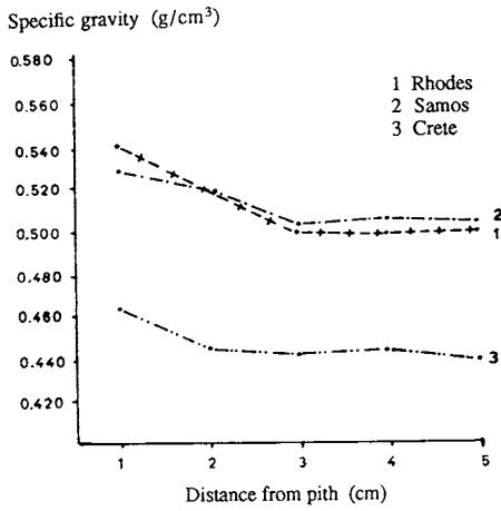
Fig. 3. Patterns of radial variation of specific gravity in the three provenances.
