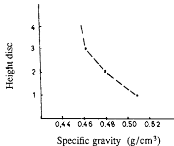
Fig. 2. Axial variation of specific gravity for Cupressus sempervirens based on 30 trees.
